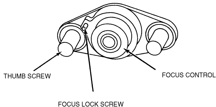
BULB ADJUSTMENT CONTROLS
